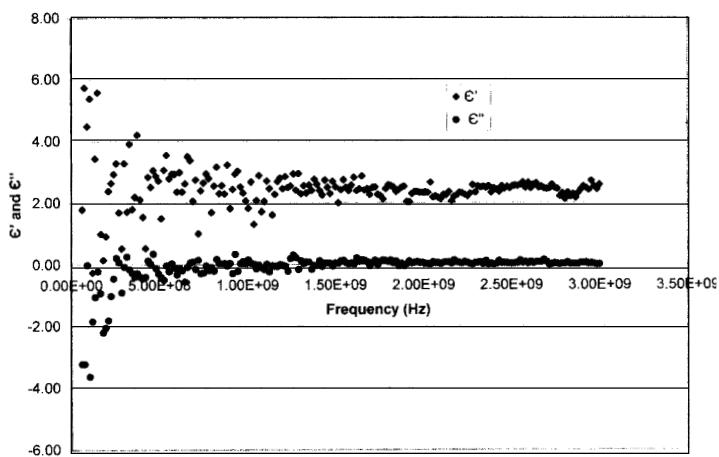
Figure-1(b): Complex permittivity Spectra of Cottonseed Oil
