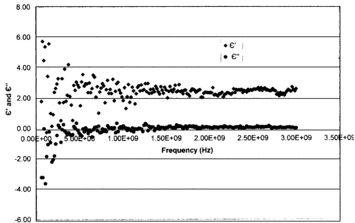
Figure-1(b): Complex permittivity Spectra of Cottonseed Oil
