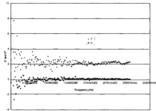
Figure-2(b): Complex permittivity Spectra of Neem Oil
