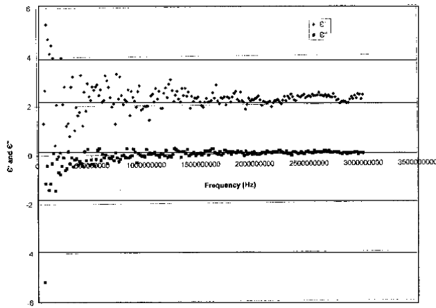
Figure-2(b): Complex permittivity Spectra of Neem Oil
