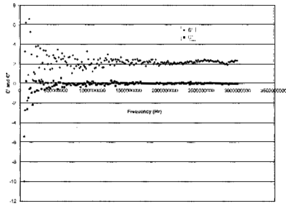
Figure-2(a): Complex permittivity Spectra of Almond Oil
