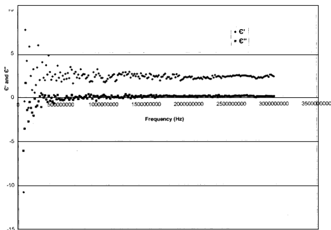
Figure-1(a) : Complex permittivity Spectra of Sunflower Oil
