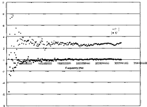
Figure-1(d): Complex permittivity Spectra of Sesame Oil
