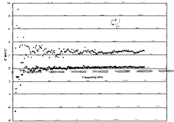
Figure-1(c): Complex permittivity Spectra of Groundnut Oil
