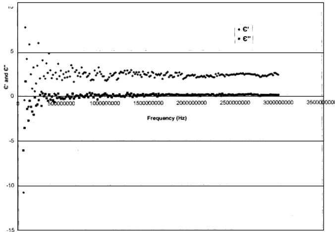
Figure-1(a) : Complex permittivity Spectra of Sunflower Oil
